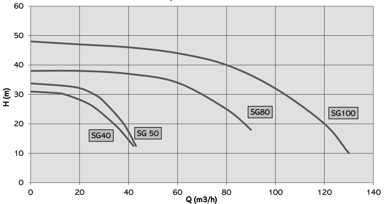
SG40-100 PP/PVDF 2900 RPM
