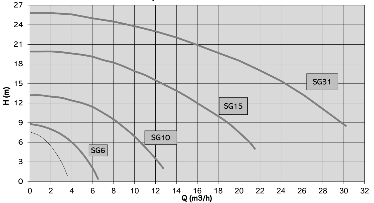
SG6-31 PP/PVDF - 2900 RPM
